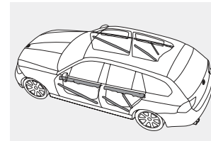
BMW's door anchoring system includes reinforcing bars with hook-like members within each door. In a serious side impact, the bars hook the door to the body, locking them together to make a more rigid passenger cell. When the pressure is released, the anchoring system is designed to disengage so that the doors can be opened (unless further damage from the impact prevents them from opening).
