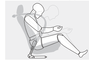
BMW restraint system for the driver and front passenger combines three-point safety belts, automatic safety-belt pretensioners, seat bolsters that help prevent occupants from sliding forward, and Active Head Restraints. This system helps provide optimum restraint in a collision.
