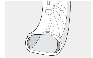
Run-flat tires allow speeds of up to 50 mph and travel from 30 to 150 miles after loss of air pressure, depending on the total vehicle weight. Reinforced sidewalls help prevent the tires from collapsing or loosening from the rim. In the event of a decline in tire pressure, the driver is warned by the Tire Pressure Monitor .
