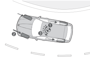
Cornering Brake Control increases vehicle stability by proportioning the braking force while turning. When you brake in a turn, the pressure comes off the rear wheels, which causes the vehicle to swerve inward (oversteer) (1). Cornering Brake Control counteracts this action by asymmetrically adjusting brake pressure (2), creating stabilizing counter-torque (3), independently of the ABS system.
