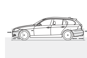
Impact-absorbing bumpers and compressible "crush tubes" front and rear help absorb the force of an impact in collisions up to nine mph, minimizing damage to the vehicle's body and simplifying repairs. Only at higher impact speeds do structural supports begin to deform, dissipating impact energy to help protect occupants.
