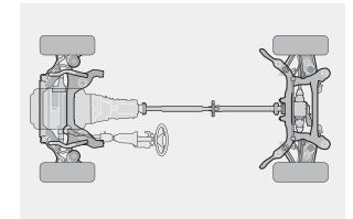
Lightweight construction is used throughout the 3 Series Sports Wagon. In both the 328i and 328i xDrive, the five-link rear suspension includes cast-aluminum upper transverse arms. In the front section of the 328i, aluminum is used extensively for suspension components, including forged-aluminum lower arms and the steering knuckle, as well as the subframe and the steering rack.
