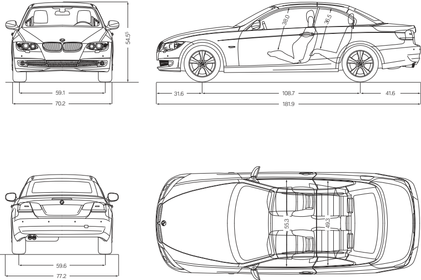
Illustrations above: all dimensions in inches.
