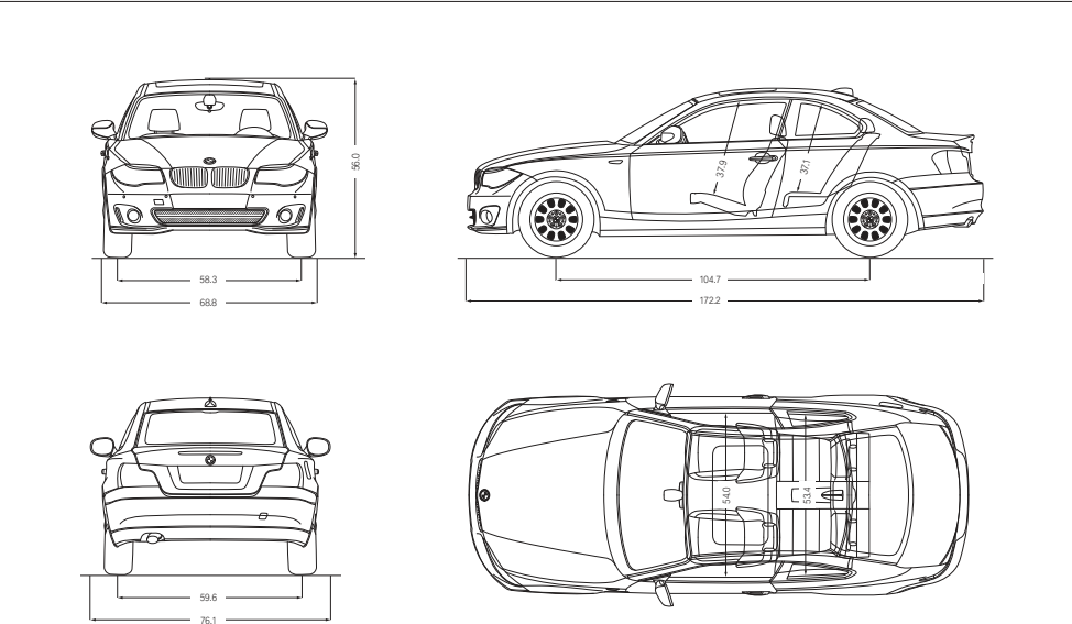
All dimensions are shown in inches and apply to 128i with standard wheels.
