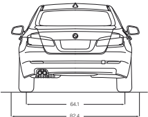
All dimensions in the technical drawings are shown in inches.
