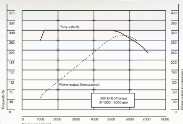
The BMW Coupe 335i with TwinPower Turbo technology: maximum output combined with minimum fuel consumption.
