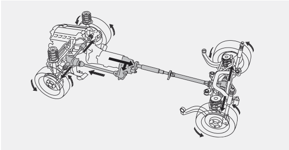
By using readings from the DSC sensors and the gas pedal, BMW's xDrive intelligent all-wheel-drive system permanently monitors the vehicle's driving condition. This data is then used to vary power distribution between the two axles, ensuring agile, neutral and forgiving handling at all times.
