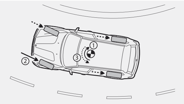
Serious drivers know: when you brake, the pressure comes off the rear wheels, causing the vehicle to swerve inward (oversteer) when turning (1). Cornering Brake Control (CBC) counteracts this action by regulating brake pressure independently of the ABS system (2), creating stabilizing counter-torque (3).
