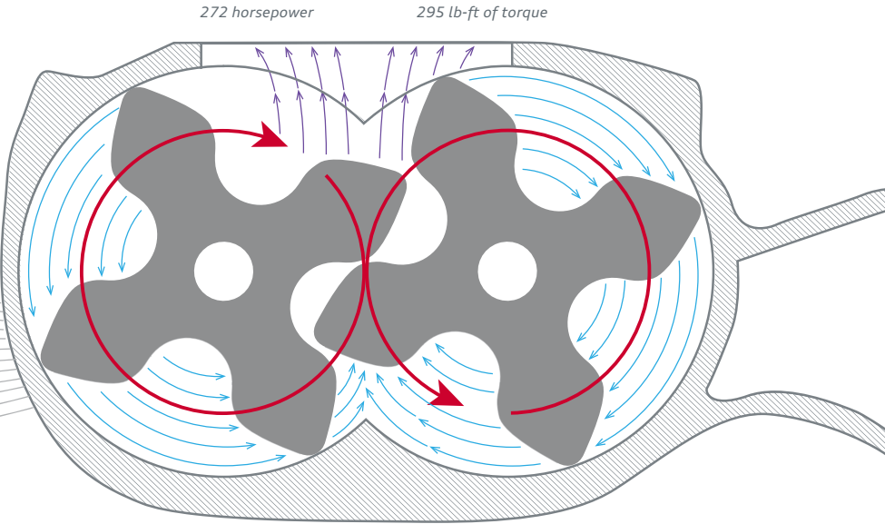
3.0 TFSI V6 supercharger illustrated above
