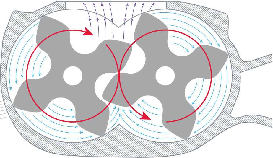
3.0 TFSI V6 supercharger illustrated above
