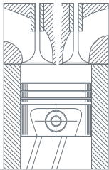
Compression
