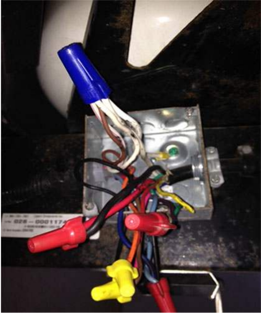
3. Poor trailer wiring connections, as shown below. General Motors does not recommend these type of connections, but many trailers utilize these connections. These type of connections are not robust and are not recommended, especially for brake wiring.
