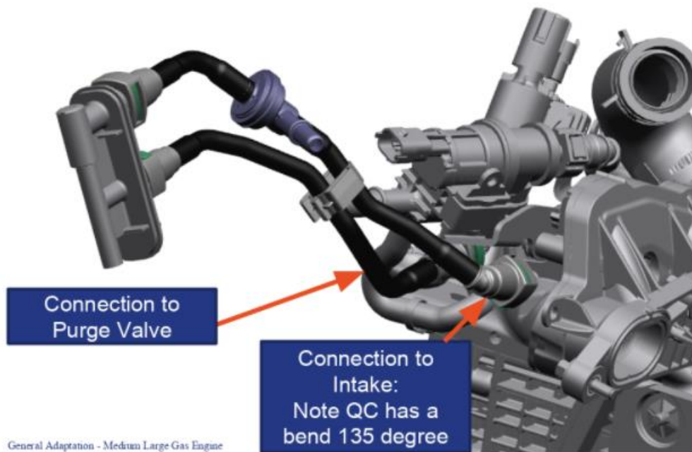
Figure 2 Lines connected to Air Box Ejector Tees and Purge Valve Port and CAC/Intake Manifold Port.
