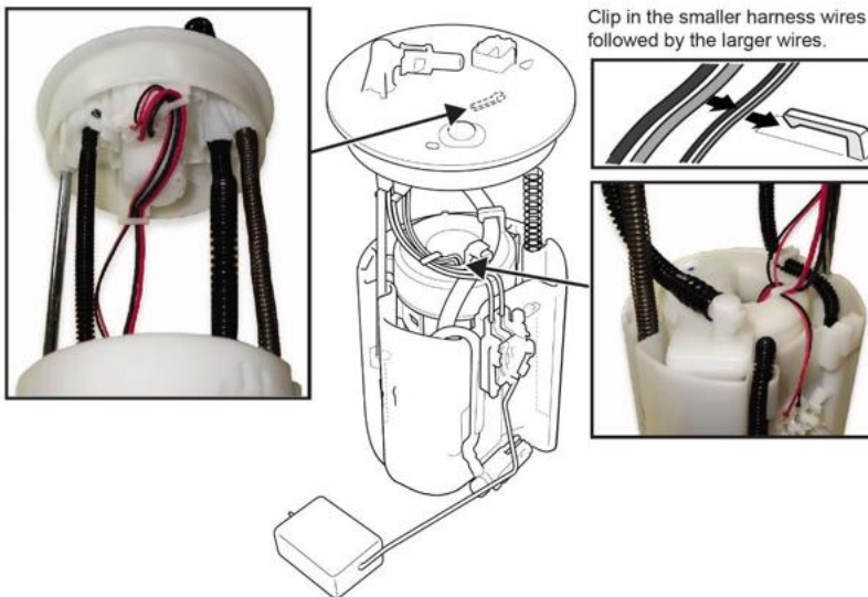
HARNESS ROUTING:
