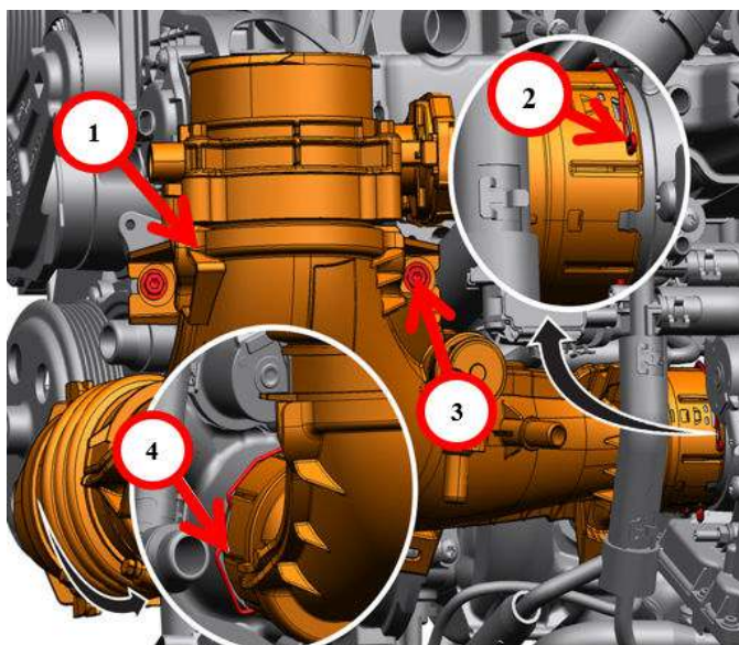
Fig. 3 Retaining Locks
