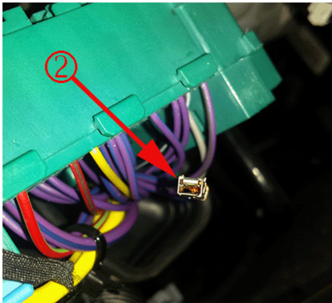
Notice terminal “spread” NO tension
