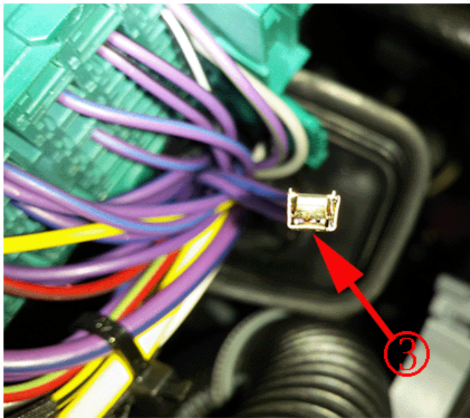
Notice Tighter tension of terminal after repair
