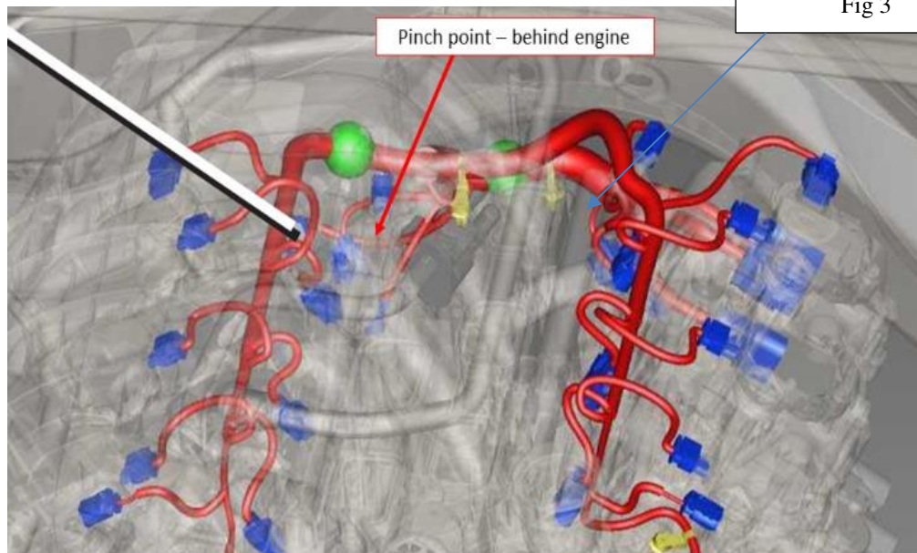
Connector Location View - SENSOR-OIL TEMPERATURE
