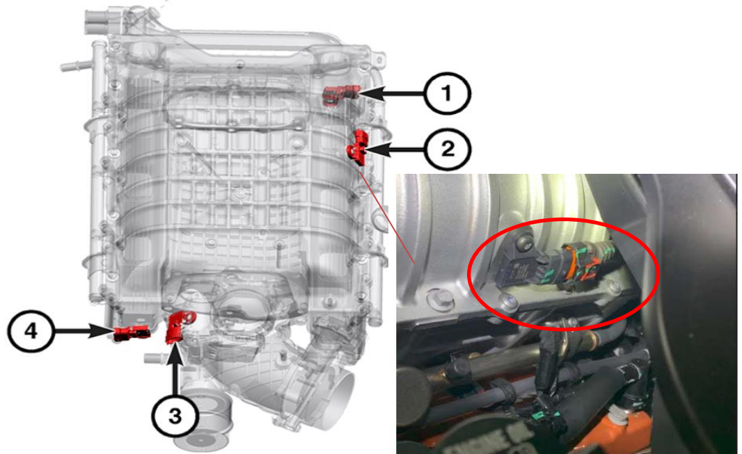
Intake TMAP Sensors
