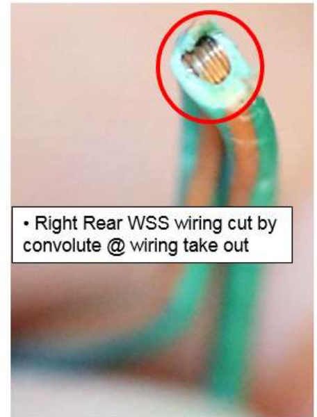
Magnified view of damaged and corroded wires near connector D1575A takeout point. Note that several strands are broken
